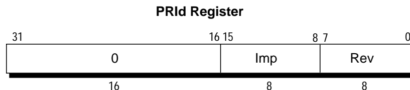
Figure 4-15 Processor Revision Identifier Register Format
