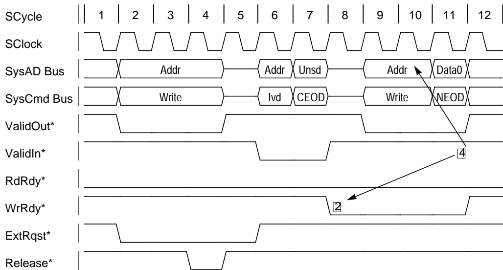
Figure 12-27 Processor Write Request Delayed for the Assertion of WrRdy* and the Completion of an External Invalidate Request
