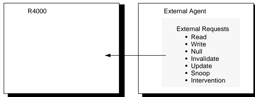
Figure 12-11 External Requests
