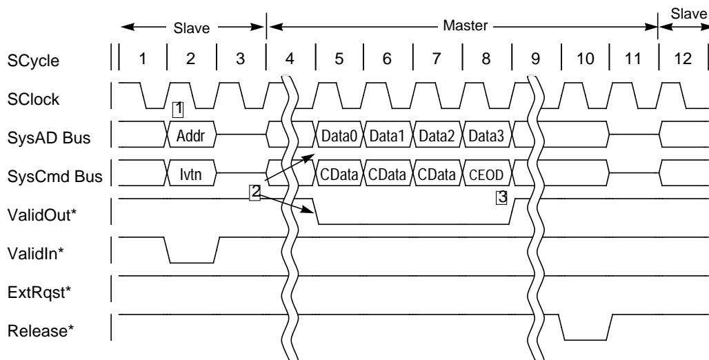
Figure 12-35 External Intervention Request, Dirty Exclusive Line, System Interface in Slave State
