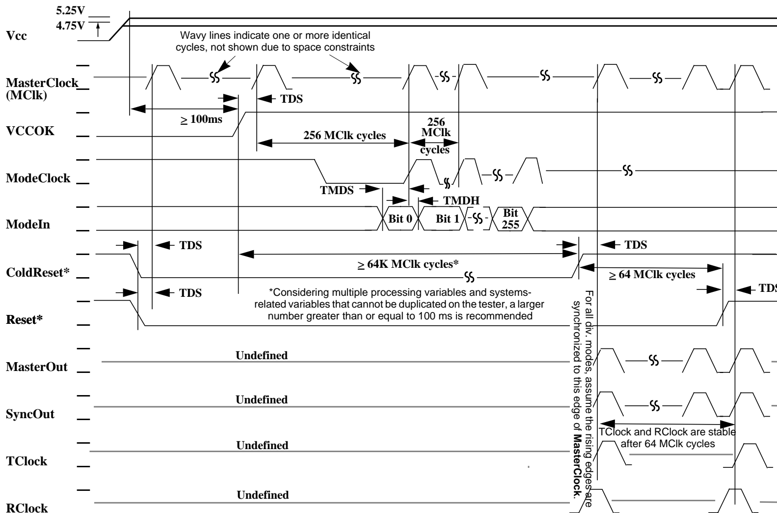
Figure 9-1 Power-on Reset
