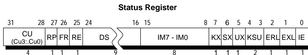
Figure 5-5 Status Register
