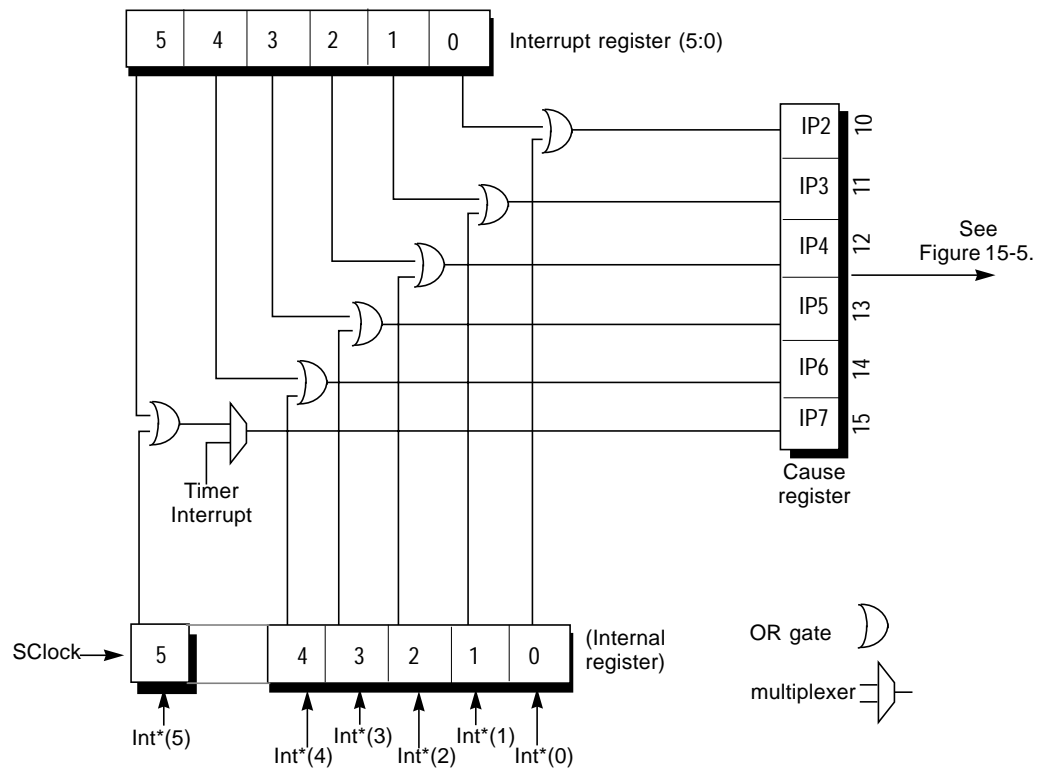
Figure 15-3 R4000PC Interrupt Signals
