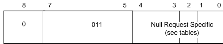
Figure 12-45 Null Request SysCmd Bus Bit Definition
