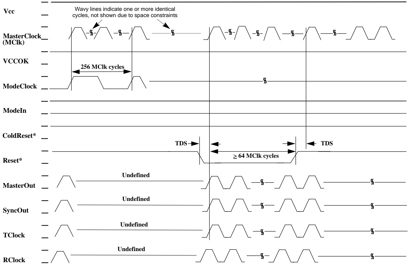
Figure 9-3 Warm Reset
