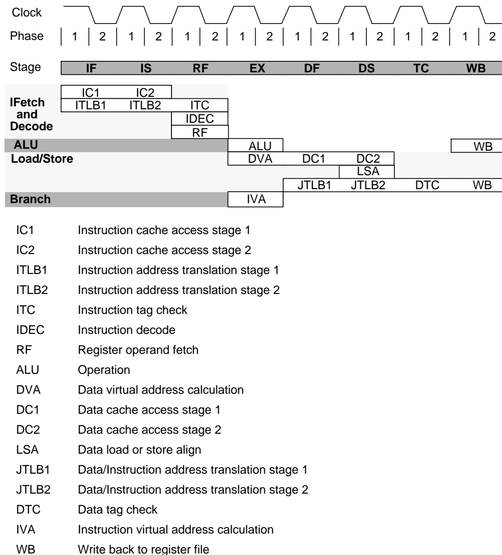
Figure 3-2 CPU Pipeline Activities
