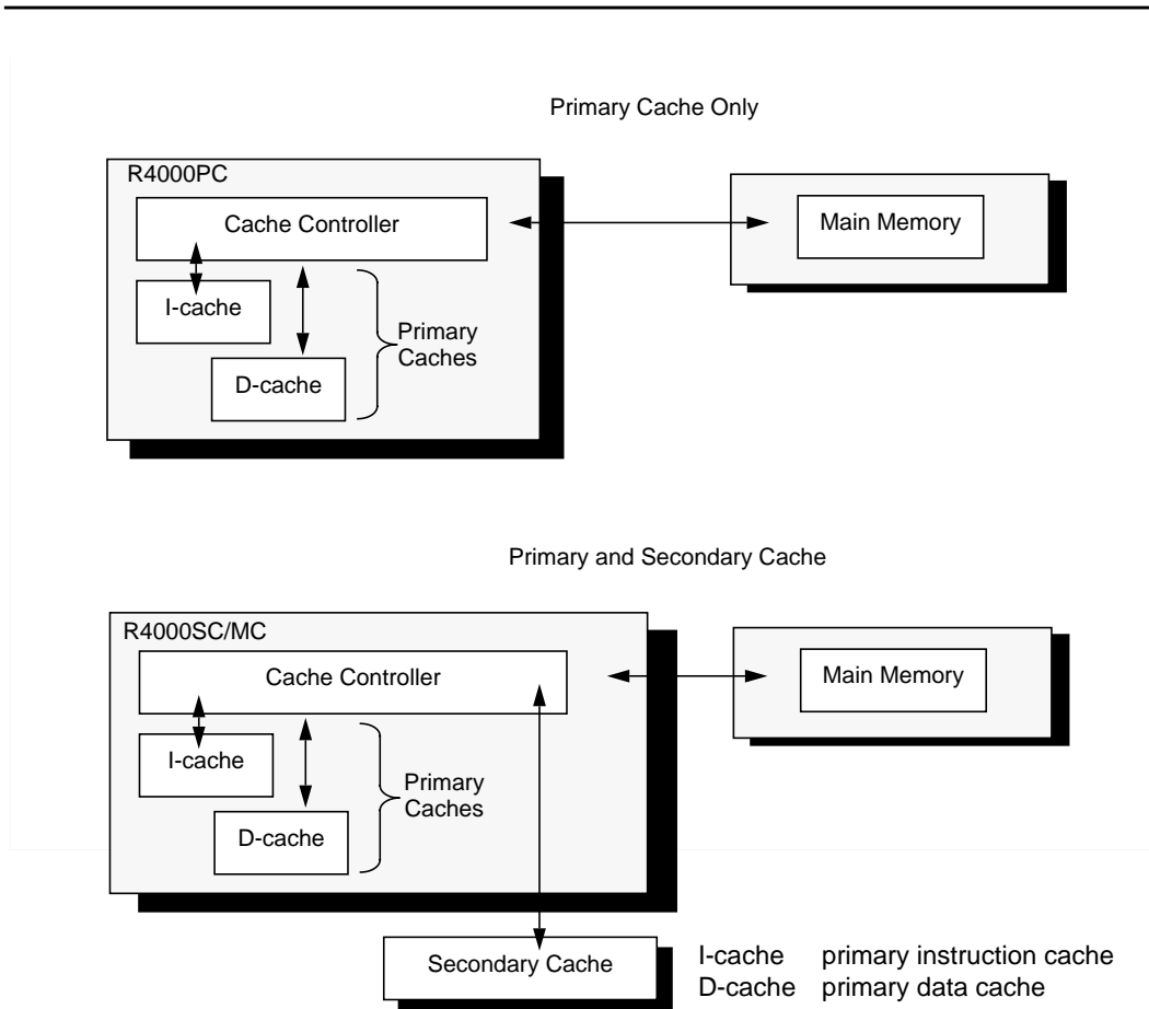
Figure 11-2 Cache Support in the R4000PC, R4000SC, and R4000MC
