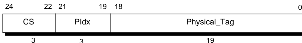
Figure 13-1 SCTag Fields
