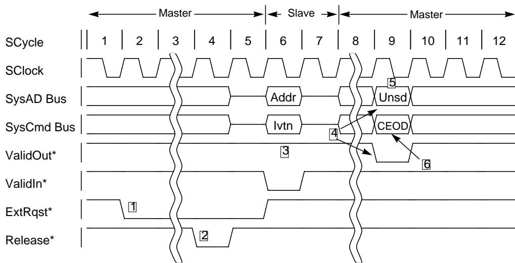
Figure 12-34 External Intervention Request, Shared Line, System Interface in Master State
