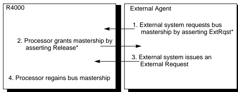
Figure 12-12 External Request
