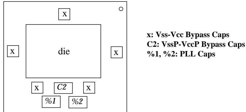
Figure E-2 179-Pin Package
